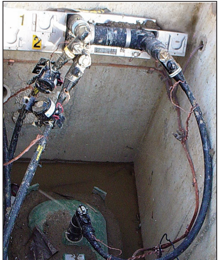
▲ Typical installation showing a 3-position feedthrough application in a submersible vault.
